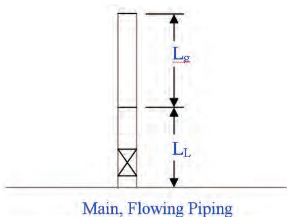
Figure 7. Liquid-Gas Stand-Pipe Used as Side Branch Absorber.
