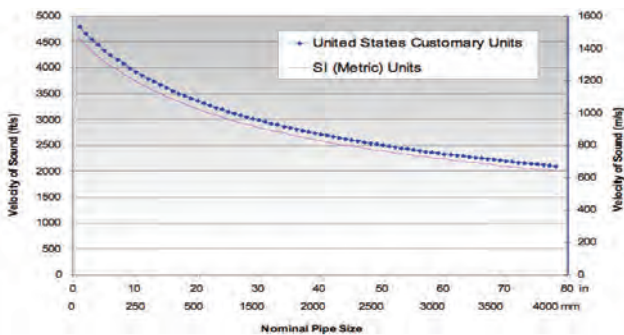
Figure 1. Graph of the Effect of Pipe Wall Compliance on Acoustic Velocity in Water (Steel Pipe, WT=0.25 inch [6.4 mm]).
