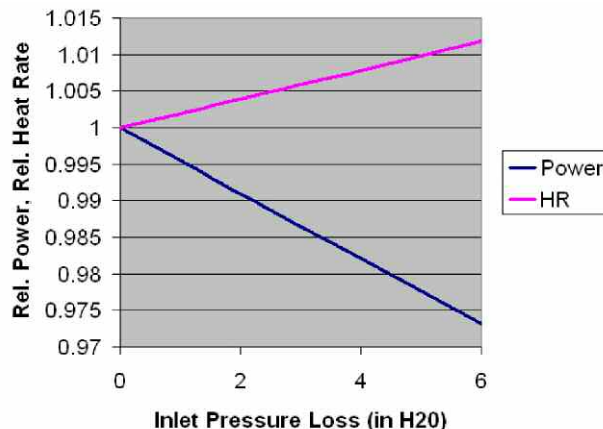
Figure 11. Impact of Inlet System Pressure Losses on Power and Heat Rate of a Typical Two-Shaft Gas Turbine.
