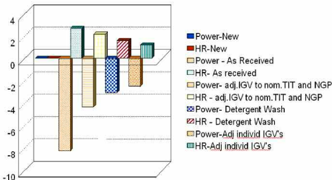
Figure 9. Performance Recovery from Sequentially Applied Methods: Adjustment of IGVs, Detergent Wash, Individual Adjustment of IGVs. (Courtesy of Kurz and Brun, 2001, ASME)
