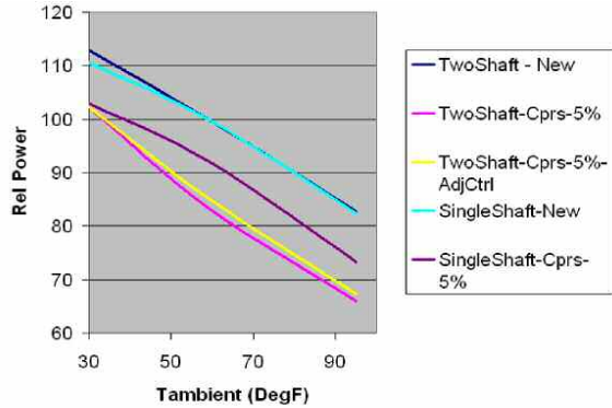
Figure 6. Impact of Loss of Compressor Efficiency Due to Degradation on Gas Turbine Power Output.
