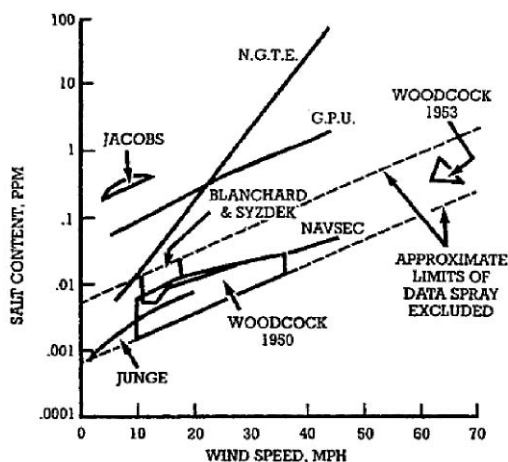
Figure 12. Salt Content in the Air in PPM as a Function of Wind Speed. (Courtesy of Cleaver, 1988, BHRA)
