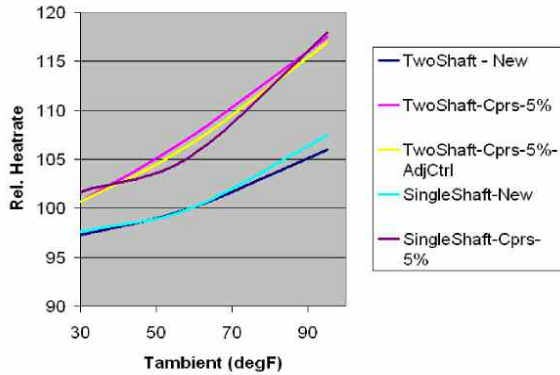
Figure 5. Impact of Loss of Compressor Efficiency Due to Degradation on Gas Turbine Heat Rate.
