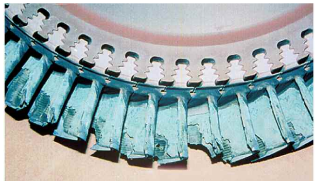
Figure 4. Hot Corrosion on a Turbine Rotor.
