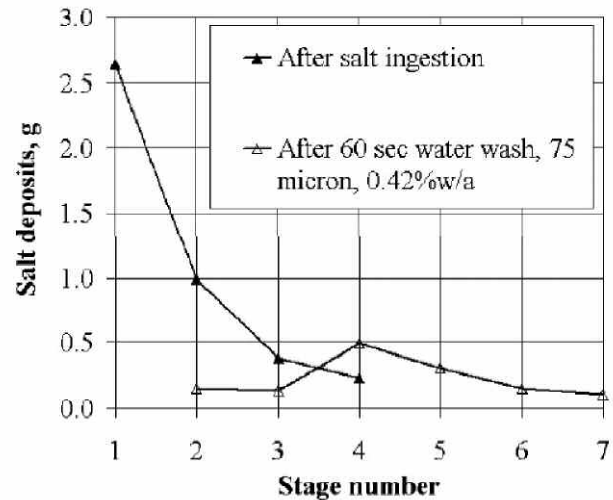
Figure 10. Salt Deposits on the Compressor Blades, Before and After Online Washing. (Courtesy of Syverud and Bakken, 2005, ASME)
