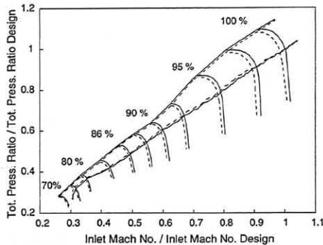
Figure 8. Comparison of a New and Clean (Solid Line) with a Degraded (Broken Line) Engine Compressor Map, and the Respective Operating Points of the Compressor. (Courtesy of Spakowszky, et al., 1999, ASME)
