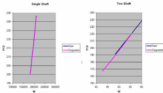
Figure 7. Gas Generator Compressor Operating Line for a New and Clean, and a Degraded Engine Compressor. (Single Shaft Left, Two Shaft Right.)
