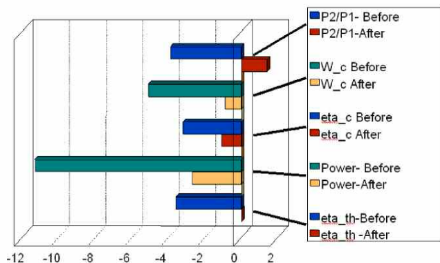
Figure 3. Performance Recovery (Compressor Pressure Ratio, Air Flow, Compressor Efficiency, Power, Thermal Efficiency) from on Crank Wash.
