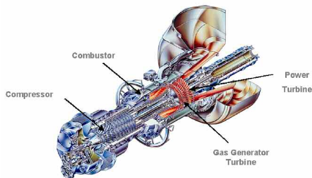
Figure 1. Typical Industrial Two-Shaft Gas Turbine.
