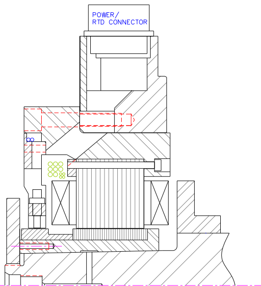
Figure 17) Shaker with Sleeve Mounted on Tapered Shaft End [9]
