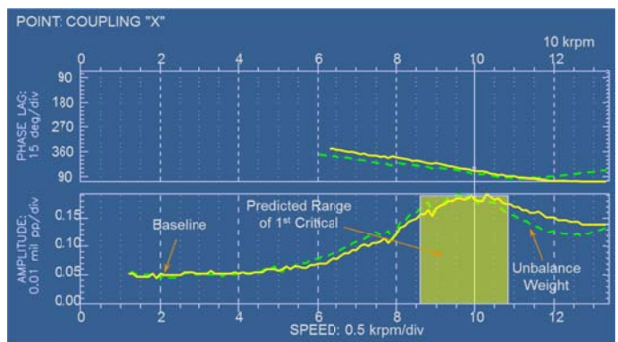
Figure 11) Measured Probe Response for 3 Stage Compressor
