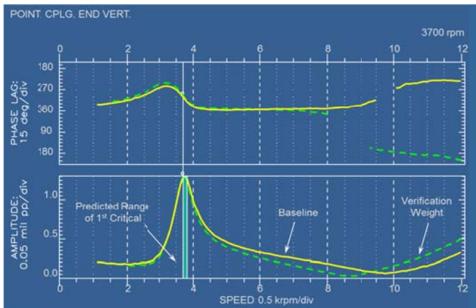
Figure 9) Measured Probe Synchronous Response for 8 Stage Compressor
