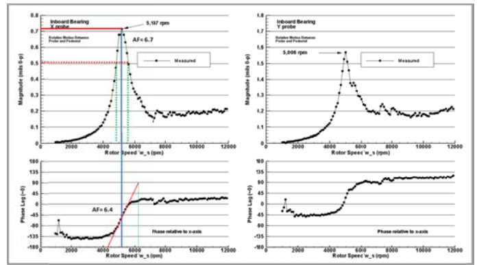
Figure 4) Bode Plot of Inboard Probe
