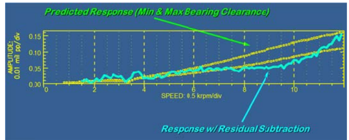
Figure 10) 8 Stage Compressor – Measured vs. Predicted Verification Response
