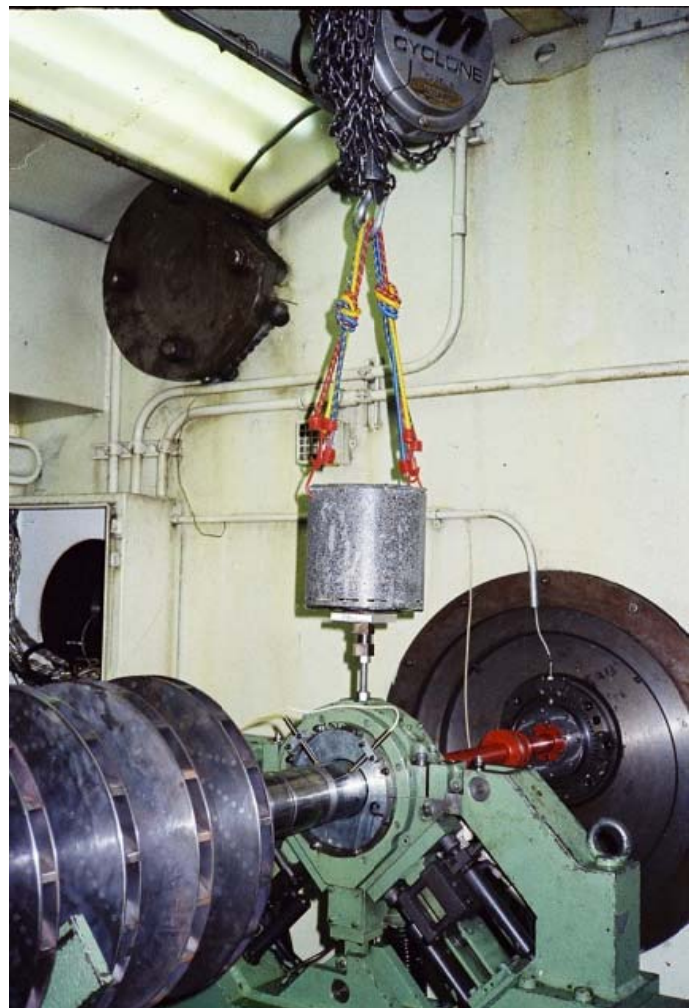
Figure 15) Shaker Mounted on Bearing Pedestal in Balance Bunker [4]
